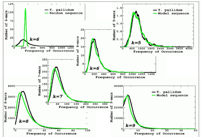
Figure 2: Comparison of k -mer distributions, k=5 to 9. Abscissa give the frequency of occurrence of a k -mer; ordinates give the number of k -mers having a given frequency of occurrence. Black: the distribution from the genome of T. pallidum ; Gray (or green): the distribution from the simulated model sequence. Top-left panel: T. pal. and random sequence, k=6 . Other panels: T. pal. and model sequence.
