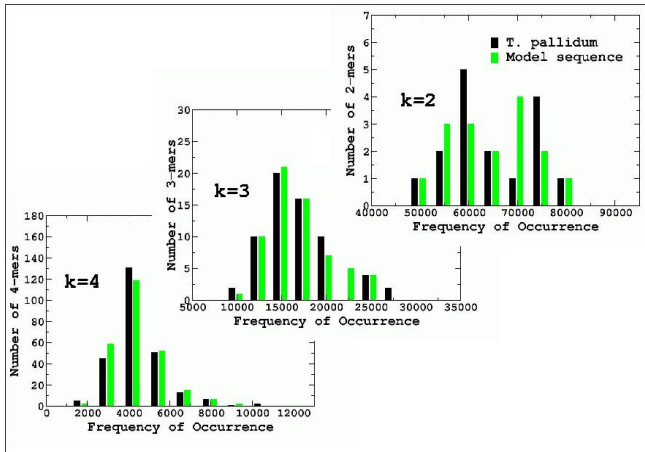
Figure 1: Histograms of k -mer distributions of genome of T. pal. (black) and model sequence (gray/green), k=2 to 4. Abscissa indicate intervals of frequency of occurrence of k -mers; ordinates give the number of k -mers falling within a given interval of frequency of occurrence. In each case the histogram of the distributions for a random sequence would be represented by a single tower located at the mean frequency.
