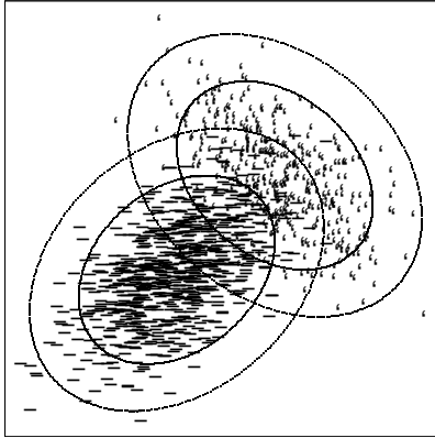
Figure 2. The synthetic data. The left bottom component consists of 800 points. The right upper component consists of 400 points. The inner and outer contours are 2\sigma contour and 3\sigma contour, respectively.
