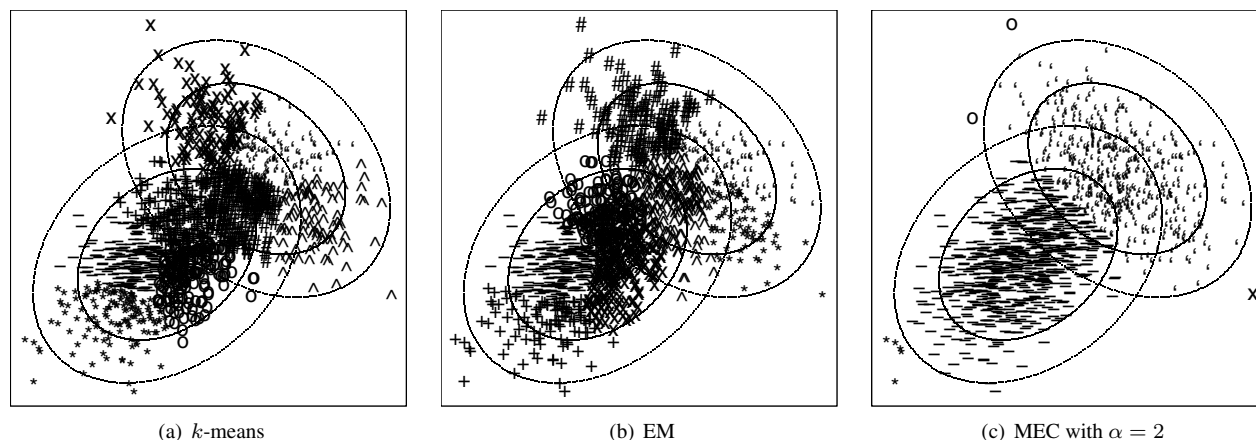
Figure 3. The clustering results on synthetic data when the specified number of clusters is 8.
